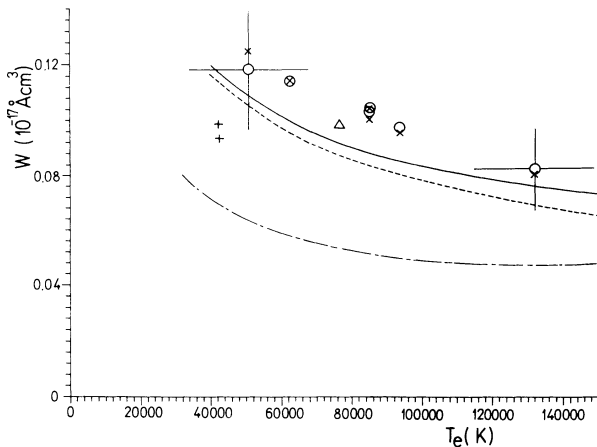
FIG. 3. Same as in Fig. 2 but for O IV 3p^2P^o - 3d^2D multiplet. Experimental results of this work: ×, 3403.56 Å and ○, 3411.76 Å.
